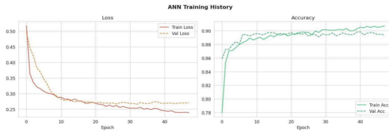
Figure 8: ANN Training History – Loss Curves (Left) and Accuracy Curves (Right)
