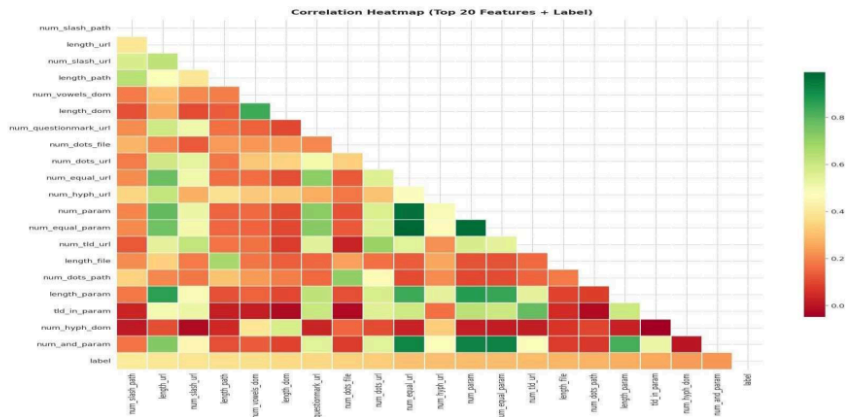
Figure 4: Correlation Heatmap of Top 20 URL Features + Target Label
