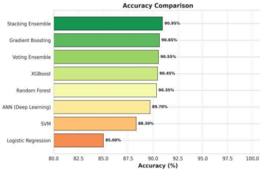
Figure 9: Accuracy Comparison – All Eight Classifiers
