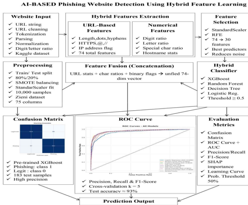
Fig. 2: Schematic Model Diagram of the Proposed Model The seven stages of the pipeline are:
