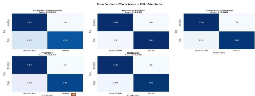
Figure 6 : Confusion Matrices — Logistic Regression , Random Forest , Gradient Boosting , SVM and XGBoost
