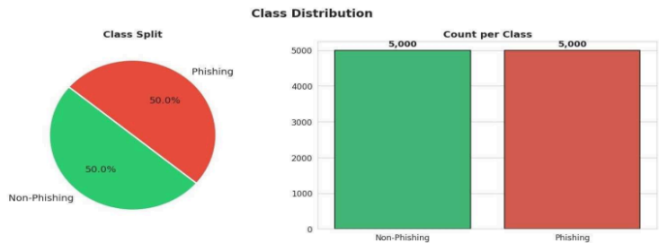
Figure 3: Class Distribution – 5,000 Phishing vs 5,000 Non-Phishing URLs (Perfect 50/50 Split)
